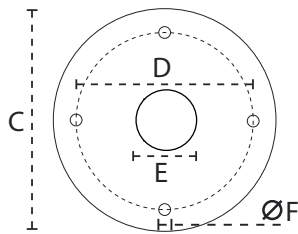
Fixed spigot for ground mounting
